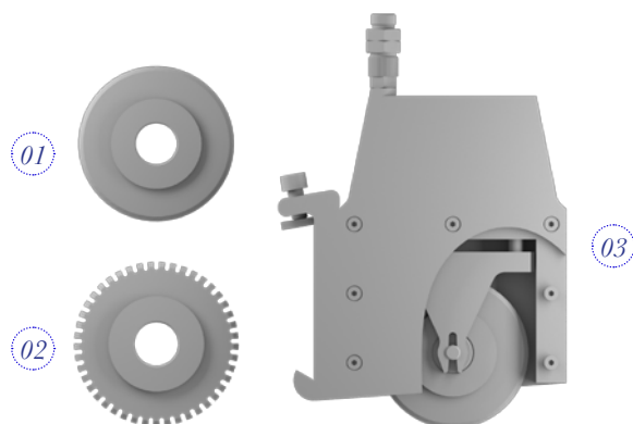
1 / Crush knife 2 / Perforating knife 3 / Pneumatic knife holder
