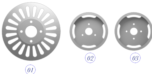
1 / Meule Ø153 2 / Meule Ø100 B64 - 3 trous 3 / Meule Ø100 B64 - 4 trous
